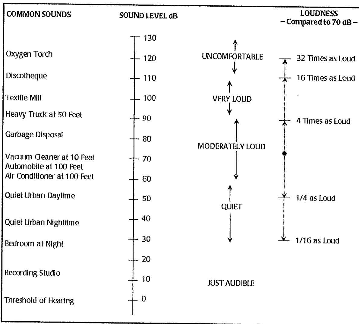
Figure G-2. Typical A-weighted Sound Levels of Common Sounds
